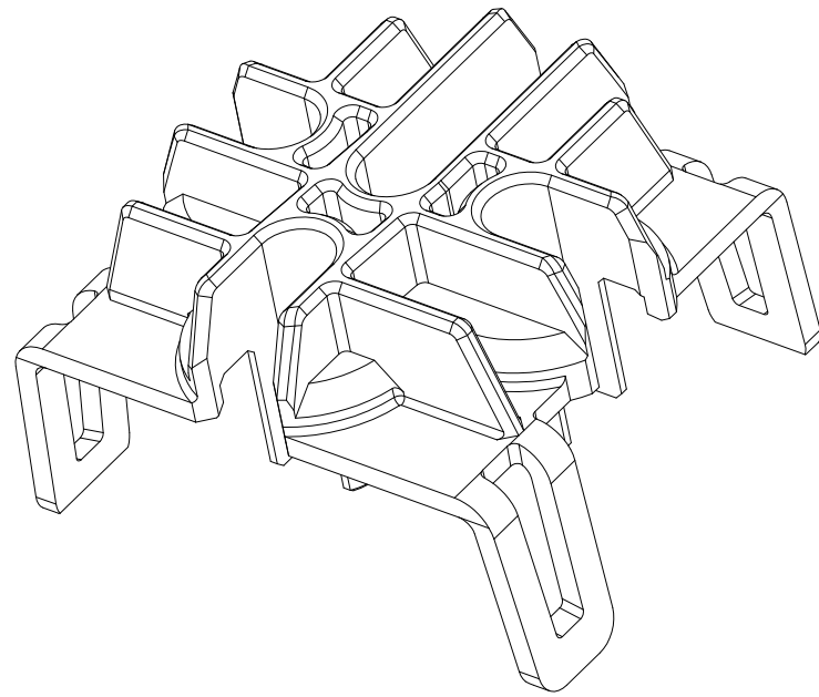
ISO VIEW FOR REF. ONLY SCALE 2:1
