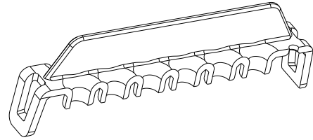
SC38-2000A-B003 TPA - PDM-S, 280 TERM (USE 6 PER ASSY FOR SC42-2005A-B001 OR 5 PER ASSY FOR SC42-2005B-B001) SCALE 1:1
