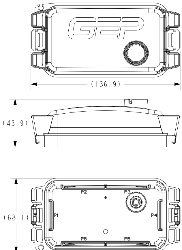
SC42-2019A-A001 COVER WITH GORE VENT - PDM-S - GEP
