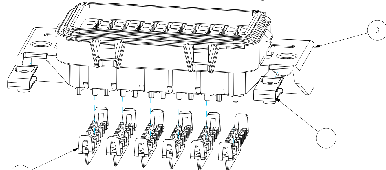
EXAMPLE CONFIGURATION EXPLODE VIEW
