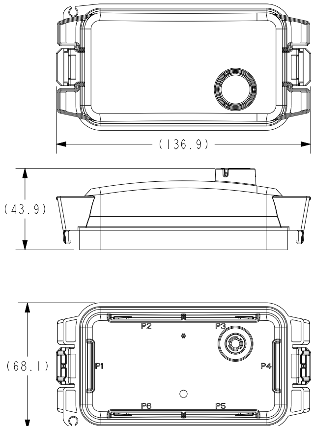
SC42-2016A-A001 COVER WITH GORE VENT - PDM-S - PLAIN
