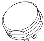
SC46-2000B-A000 GORE VENT (INCLUDED WITH SC42-2016A-A001 & SC42-2019A-A001) SCALE 1:1
