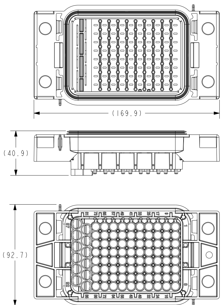
SC42-2008B-B001 HOUSING AND SEAL - PDM-U, 92 POS, 280 AND ATO TERM, 10MM SEE NOTE 5
