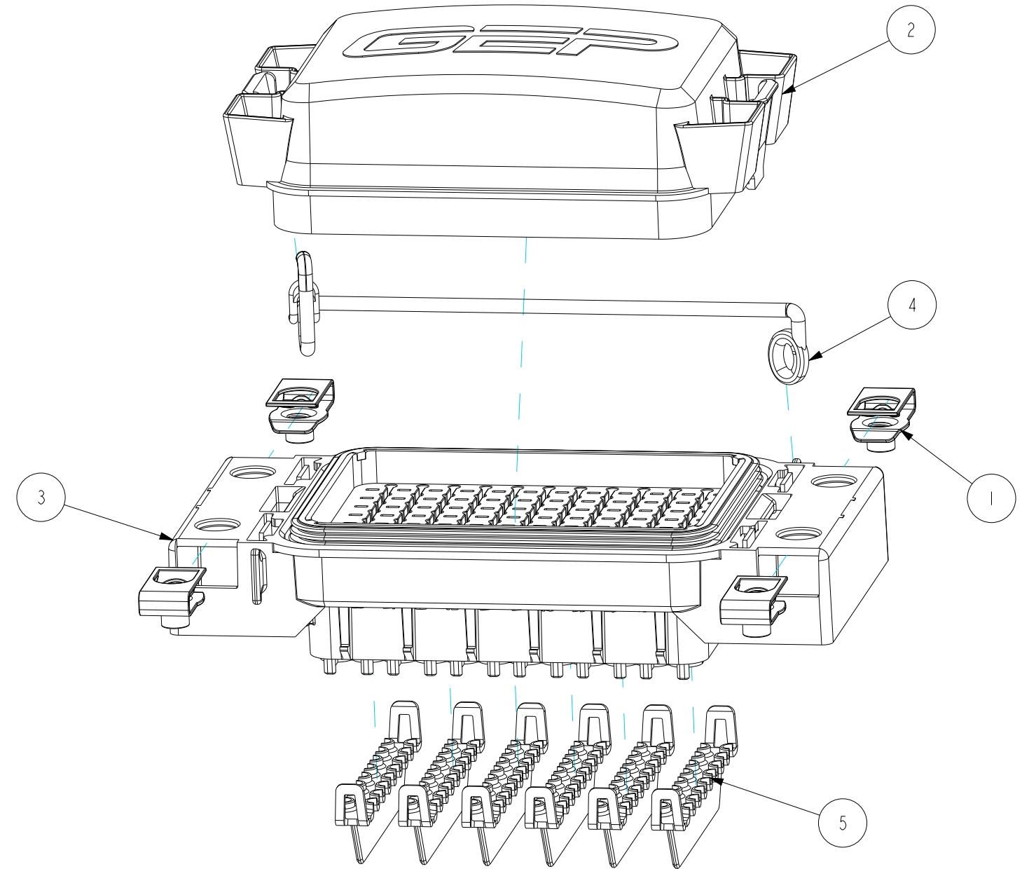
EXAMPLE CONFIGURATION EXPLODE VIEW
