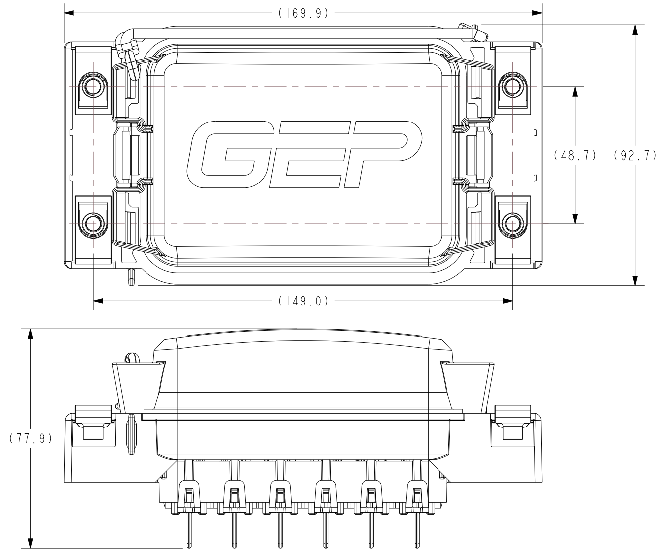
EXAMPLE CONFIGURATION WITH DIMENSIONAL INFO
