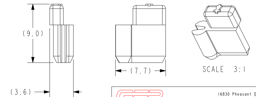
PDM-TK DIODE KEY
