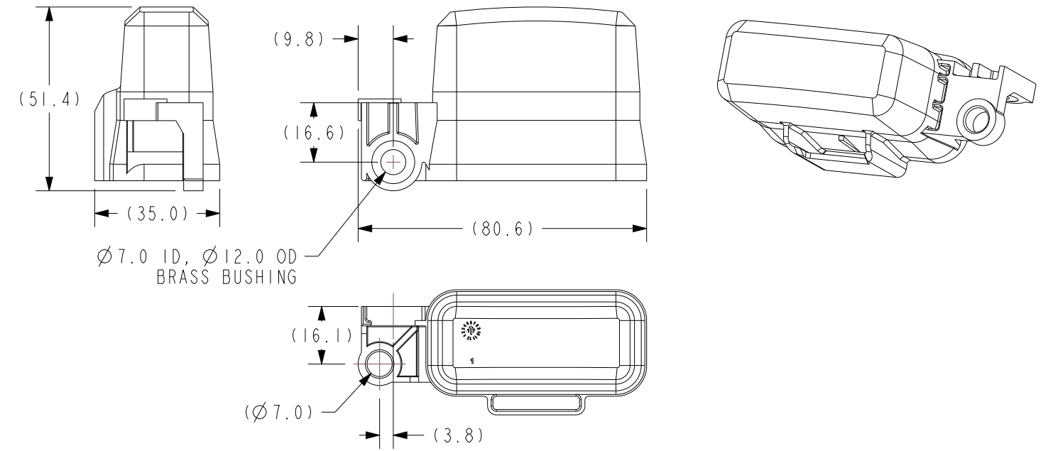
FRH-A12-CB-1 COVER - PDM, FRH 12 POS, SINGLE SIDE MOUNT, PLAIN
