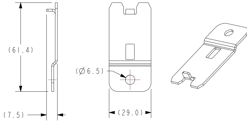
FRH-A12-MB-A1 BRACKET - PDM,FRH,FLAT WITH ANTI-ROTATION, ZINC STEEL
