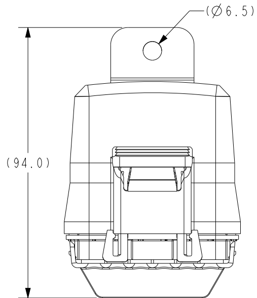
EXAMPLE CONFIGURATION WITH DIMENSIONAL INFO
