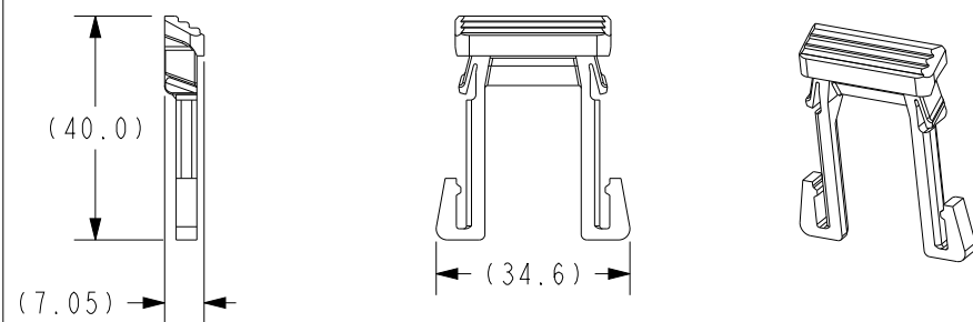
FRH-A-CPA CPA - PDM, FRH
